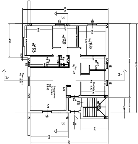
Piano terra
